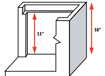
INTERNAL VIEW
