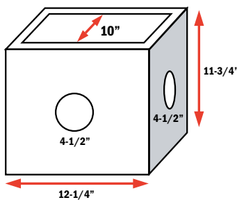
SIDES 1 & 2
