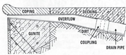
TYPICAL INSTALLATION
