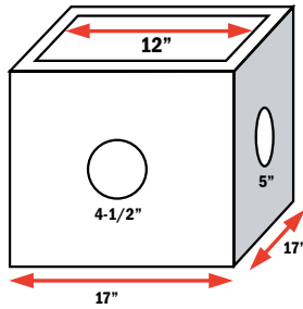
SIDES 3 & 4
