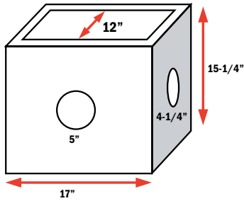
SIDES 1 & 2
