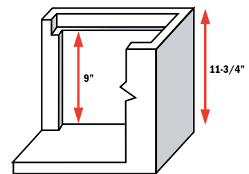
INTERNAL VIEW
