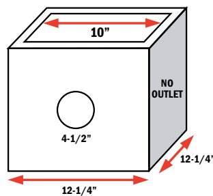
SIDES 3 & 4
