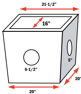
SIDES 3 & 4
