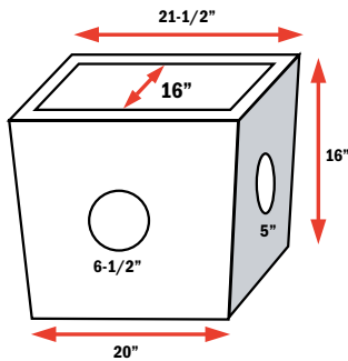
SIDES 1 & 2
